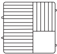
Plate Rack w/4 Extenders No. PM2110-4 Plate - D8 3 / 4 to D9 9 / 16 Max. H1 Cap. 21 2 pcs./14# • 4.3 cu.ft.
