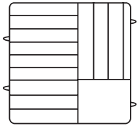
Plate Rack w/5 Extenders No. PM1211-5 Plate - D9 9 / 16 to D10 3 / 4 Max. H1 1 / 4 Cap. 12 2 pcs./27# • 5.5 cu.ft.
