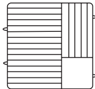
Plate Rack w/6 Extenders No. PM2011-6 Plate - D10 3 / 4 to D11 Max. H1. Cap. 20 1 pc./14# • 3.3 cu.ft.
