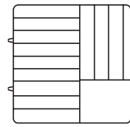
Plate Rack w/4 Extenders No. PM1211-4 Plate - D8 3 / 4 to D9 9 / 16 Max. H1 1 / 4 Cap. 12 2 pcs./15# • 4.3 cu.ft.
